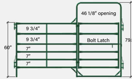
5' High Corral Panel - 6 Bar with Gate
