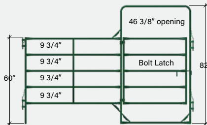
5' High Handy Panel - 5 Bar with Gate
