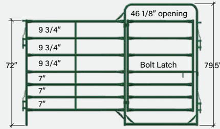
6' High Corral Panel - 7 Bar with Gate
