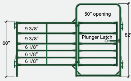
5'h Heavy Duty Panel - 6 Bar w Gate
